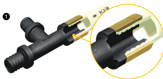
1. Cross-section of a Push joint.
